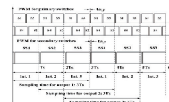
[ PWM scheme for the Multiple Output Charger ]
