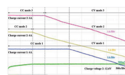
[ Charge profiles of the three batteries being charged by the proposed Multiple Output Charge ]
